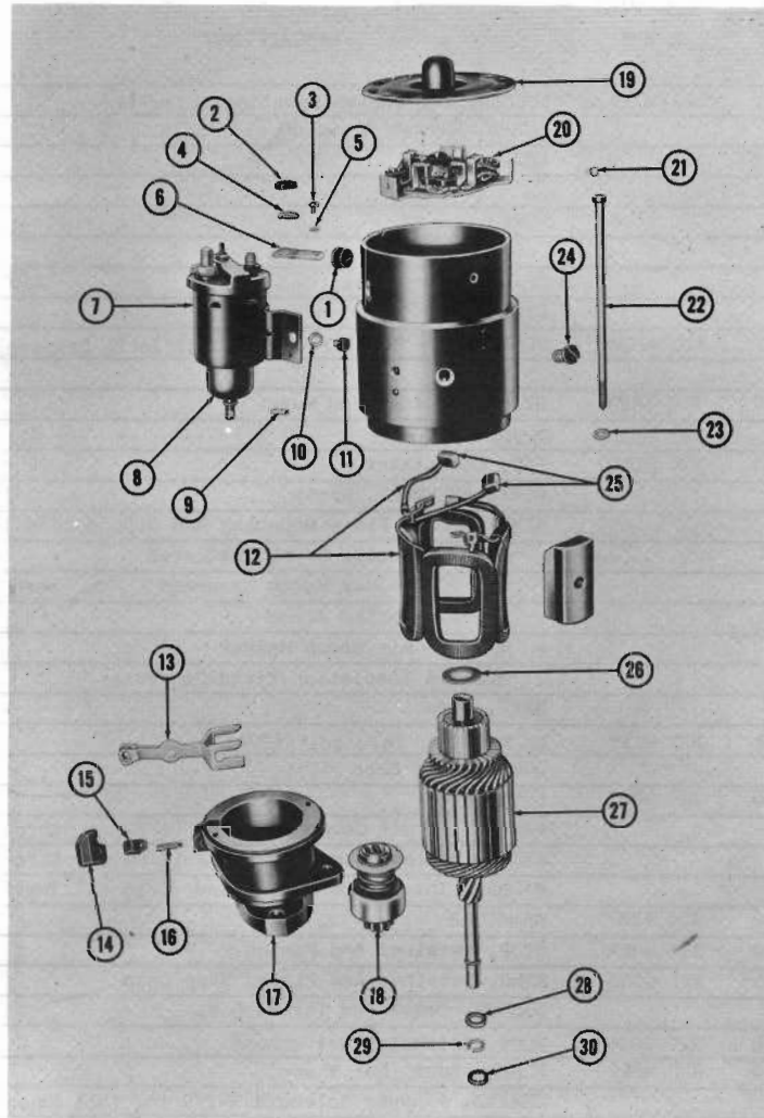
STARTING MOTOR 164-165 10-80 (V8)
