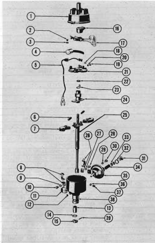
DISTRIBUTOR 164-165 01 (LHE)
