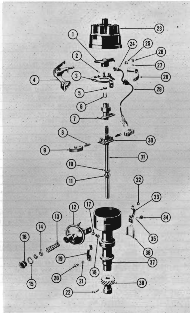
DISTRIBUTOR 164-165 10-80 (V8)
