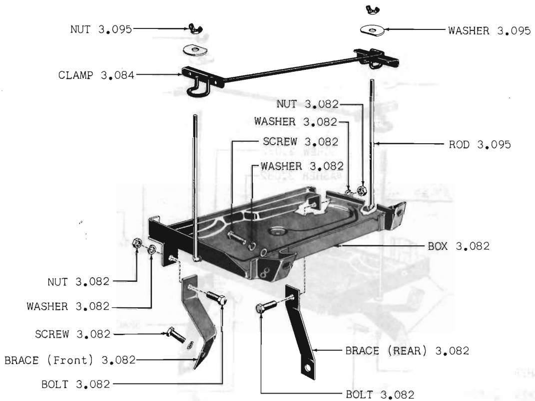
BATTERY BOX 60-61 10
