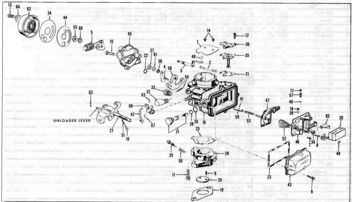
CARBURETOR 61-62 10 (WST-LDT)(WOD-LDT)
