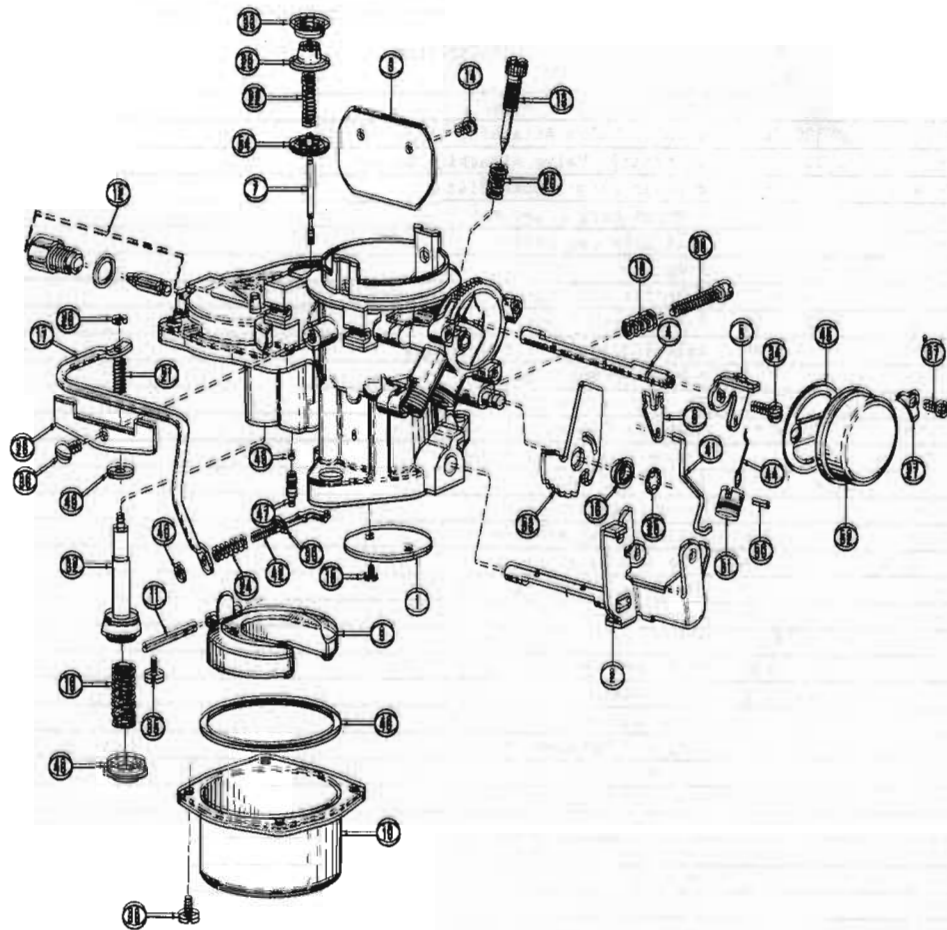
CARBURETOR 65 01-10 (GHV-100-LDT)
