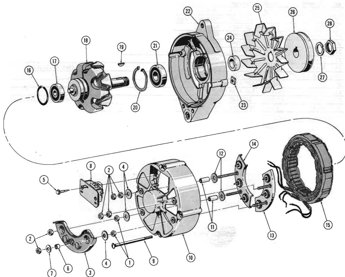
ALTERNATOR (Less Pulley and Belt)(40 AMP.) 64-65 01-10-80
